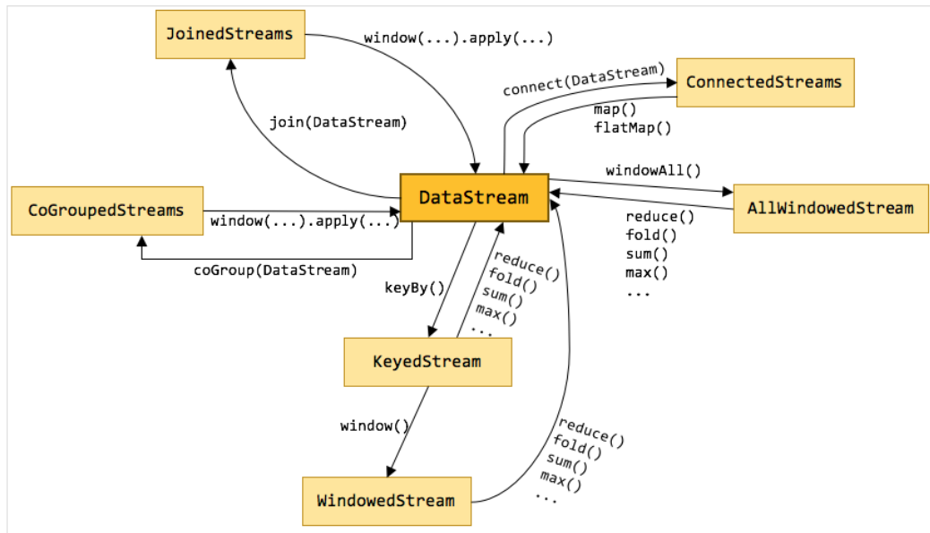
Figure 8-63 Conversion of Flink stream types
