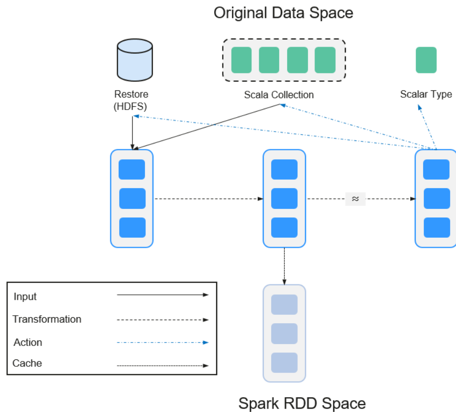
Figure 24-2 RDD operation
