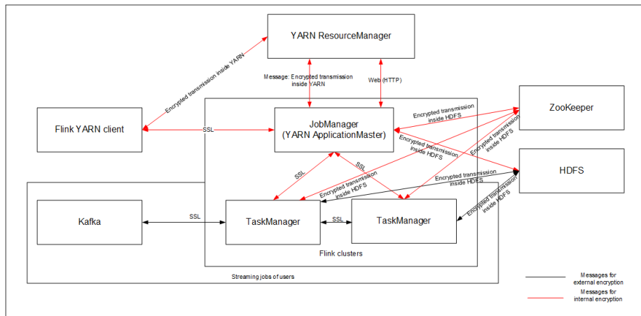
Figure 8-34 Encrypted transmission of Flink
